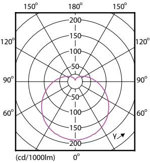
Light Distribution Diagram - EcoHome LEDBulb 13W E27 6500KHV 1PF/20AR
