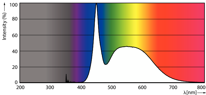
Spectral Power Distribution Colour - LEDBright 20W E27 6500K HV 1PF/12 AR
