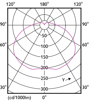
Light Distribution Diagram - LEDBright 20W E27 6500K HV 1PF/12 AR
