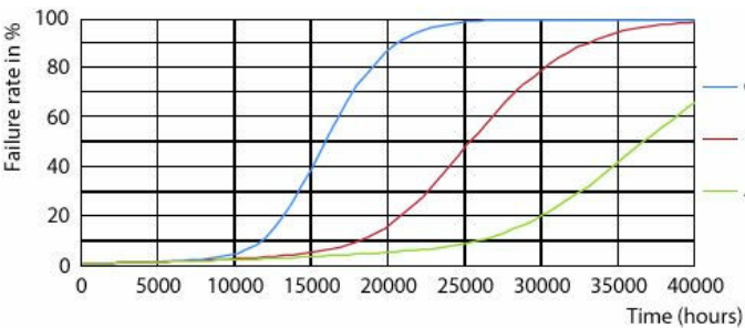
LEDtube 25K FailureRate
