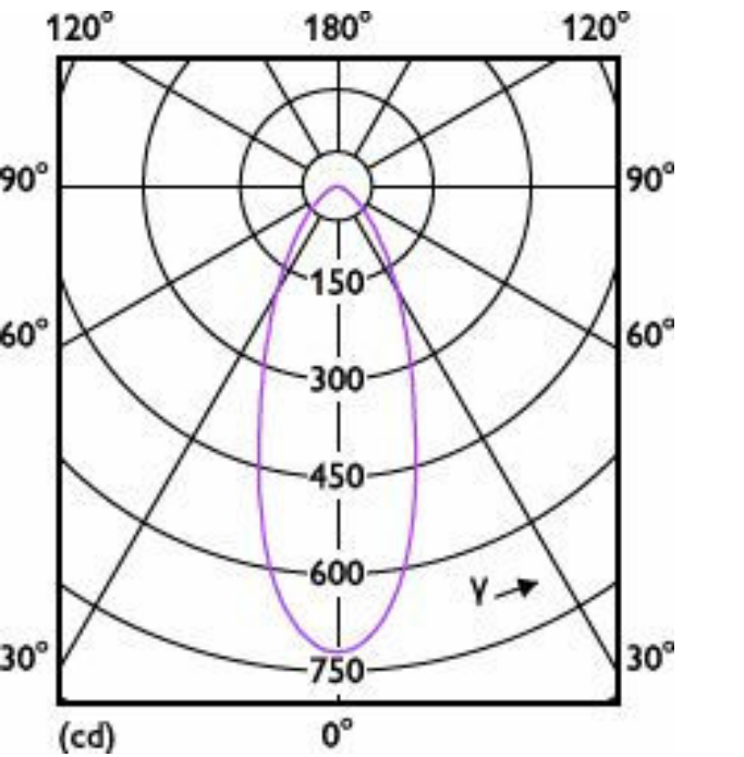
Light Distribution Diagram - SL052 RD SPOT 070 6.2W 27K WH WW
