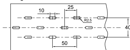
Large Duct
