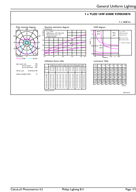
General uniform lighting - Ecofit E Mains 1200mm 16W 765 T8
